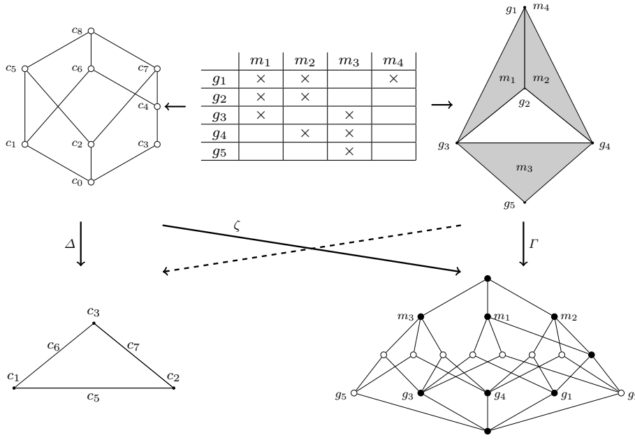
Fig. 1 In the upper part of the diagram one finds a formal context (center), the associated concept lattice (left) and the associated simplicial complex (right). The formal concepts of the concept lattice are given as c_0 = (\emptyset, \{m_1, \dots, m_4\}) , c_1 = (\{g_3\}, \{m_1, m_3\}) , c_2 = (\{g_4\}, \{m_2, m_3\}) , c_3 = (\{g_1\}, \{m_1, m_2, m_4\}) , c_4 = (\{g_1, g_2\}, \{m_1, m_2\}) , c_5 = (\{g_3, g_4, g_5\}, \{m_3\}) , c_6 = (\{g_1, g_2, g_3\}, \{m_1\}) , c_7 = (\{g_1, g_2, g_4\}, \{m_2\}) and c_8 = (\{g_1, \dots, g_5\}, \emptyset) . In the simplicial complex filled triangles correspond to 2-dimensional simplices while the triangle in the middle is a hole. The lower part of the diagram, in particular the meaning of \Delta , \Gamma , \zeta and the dashed arrow, is explained in Section 3.
