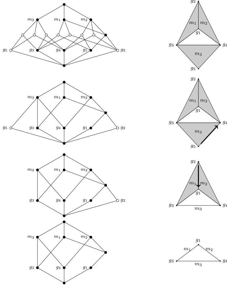
Fig. 2 The proof of theorem 1 illustrated by the example from figure 1. Left from top to bottom: Reduction of the lattice \Gamma(\mathcal{S}_{\mathbb{K}}) to the concept lattice \mathcal{B}_{\mathbb{K}} . The latter lattice can be embedded into the first via the map \zeta depicted in figure 1. The nodes in the image of this map are filled black. One passes from the uppermost to the lowermost lattice by removing maximal non-filled nodes, one at a time. — Thus in fact there should be seven steps between the first and the second lattice. Right: Each simplicial complex is the image of the lattice left to it under the map \Delta . The labels serve to retrace this association: Atoms and co-atoms of the lattices become vertices and maximal simplices of the simplicial complexes respectively. The uppermost simplicial complex is (\Delta \circ \Gamma)(\mathcal{S}_{\mathbb{K}}) = \mathcal{S}_{\mathbb{K}} , and the lowermost is \Delta(\mathcal{B}_{\mathbb{K}}) . As proved in the text for the general case, each simplicial complex is a strong deformation retract of the simplicial complex above it. An arrow indicates a retraction that will occur in the next step. The retraction should be imagined as a projection parallel to the arrow.
