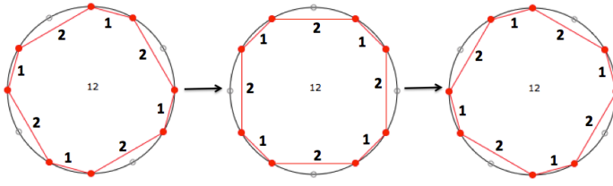
Fig. 4 A MLT whose intervallic structure is equal to (1 2 1 2 1 2 1 2), i.e. it is four times the repetition of the sub-pattern (1 2). Note that the sum of the elements of the sub-pattern is equal to 3, meaning that the associated musical object has three possible transpositions, as in the case of Fig. 3
