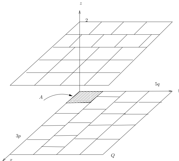
FIGURE 1. The group \mathbb{Z}_{3p} \times \mathbb{Z}_{5q} \times \mathbb{Z}_2
